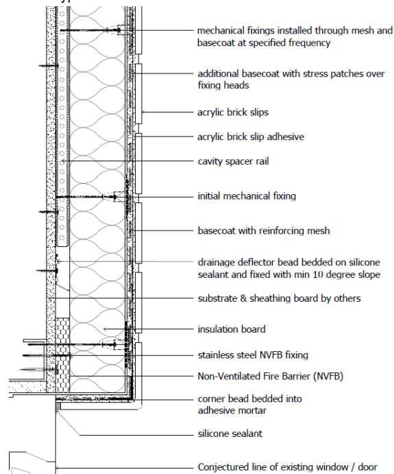
Diagram 10 - Typical window/door head detail
