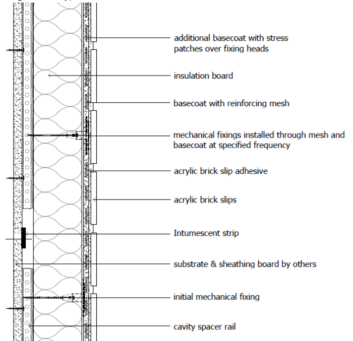
Diagram 4 - Typical horizontal fire barrier detail
