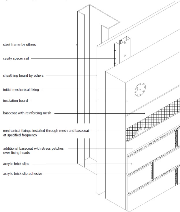
Diagram 3 - Typical build-up detail
