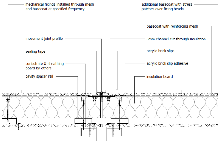
Diagram 2 - Typical movement joint detail
