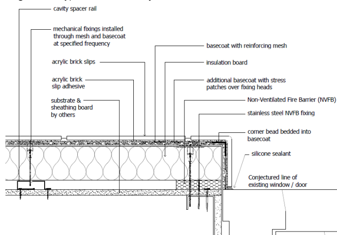
Diagram 10 - Typical window/door head detail
