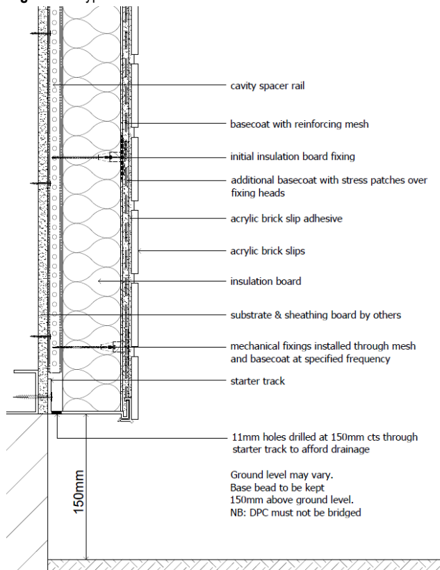
Diagram 5 - Typical base detail
