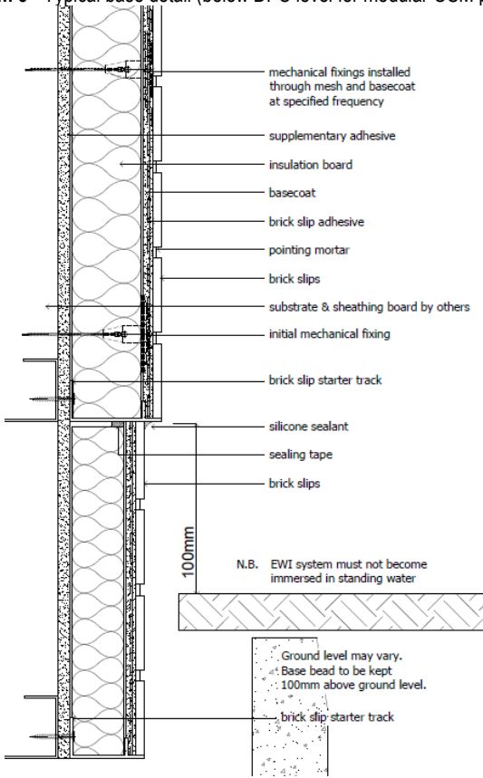
Diagram 5 - Typical base detail (below DPC level for modular OSM projects)
