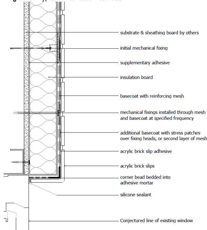
Diagram 9 - Typical window/door head detail
