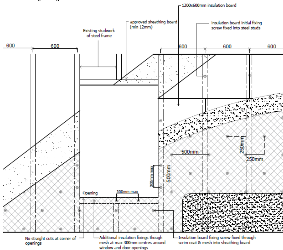
Diagram 1 - Typical mechanical fixing arrangement
