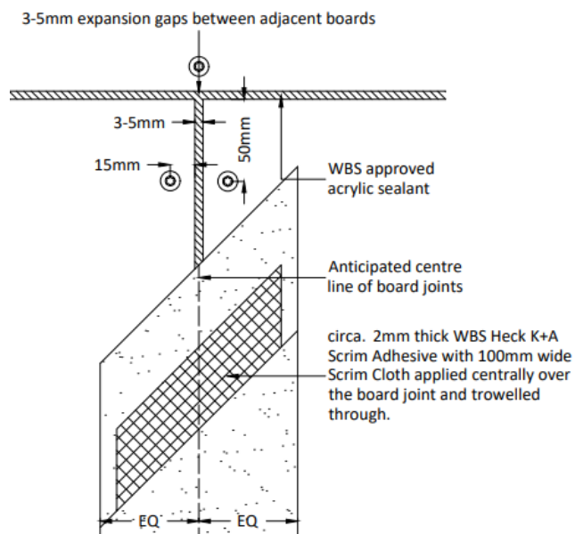
Diagram 2 - Typical carrier board junction
