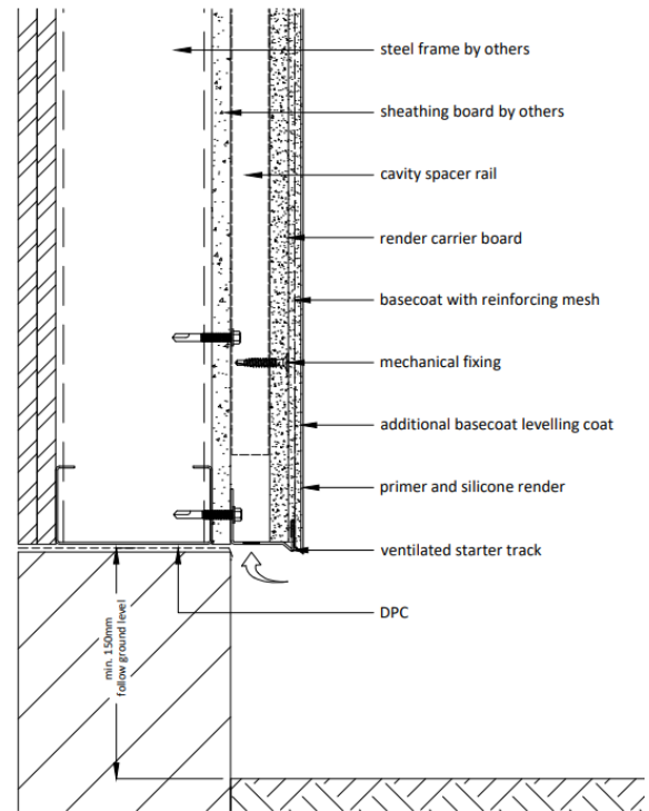
Diagram 5 - Typical base detail
