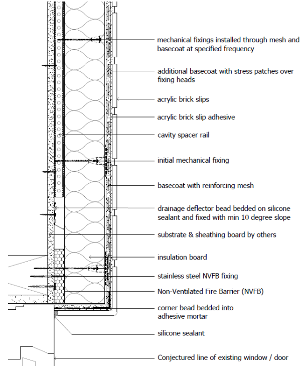
Diagram 10 - Typical window/door head detail
