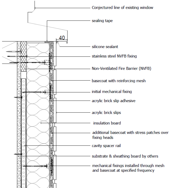
Diagram 9 - Typical window cill detail
