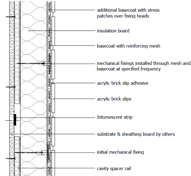
Diagram 4 - Typical horizontal fire barrier detail
