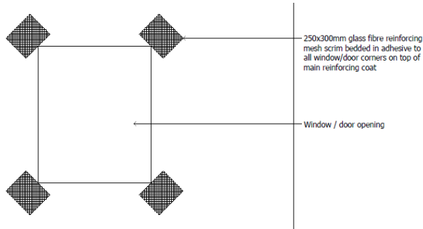
Diagram 7 - Typical opening stress patches detail
