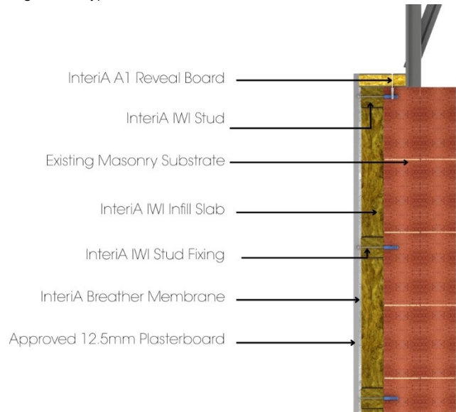
Diagram 7 - Typical external corner detail
