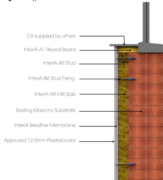
Diagram 5 - Typical reveal detail
