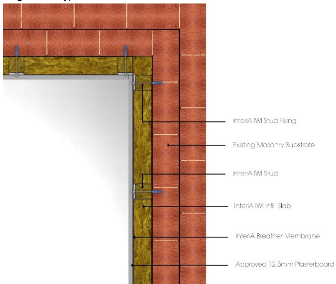
Diagram 6 - Typical internal corner detail
