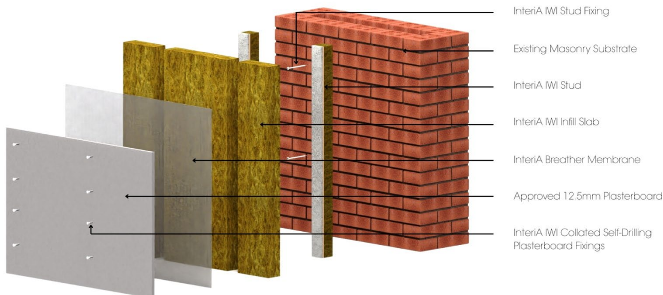
Diagram 1 - Typical build up detail of System
